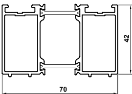
DV515 Outer Frame Extension
