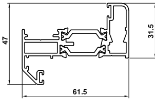
ETC321 Externally Glazed Sash System 2
