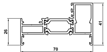
ZSB169 Outer Frame
