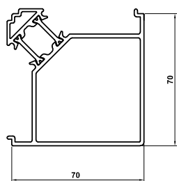
ETC048 Corner Post
