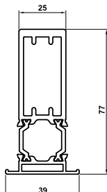
ETC517 Coupler
