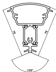
ETC385 135° Corner Post
