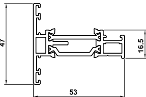
ETC324N Internally Glazed Slimline Sash System 1
