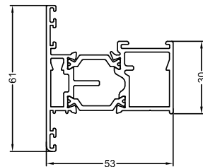
ETC424N Internally Glazed Medium Sash System 1
