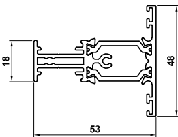
ETC333 T-Transom/Mullion
