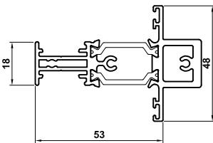
ETC336 T-Transom/Mullion
