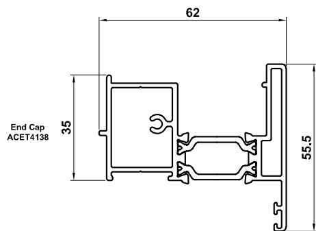
ETC4138 French Casement Mullion
