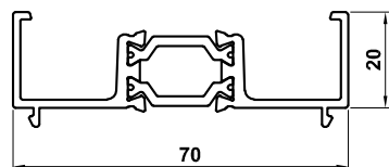
DV559 Outer Frame Extension
