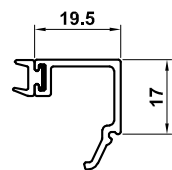
UN3160G 28mm Glazing Bead with Gasket
