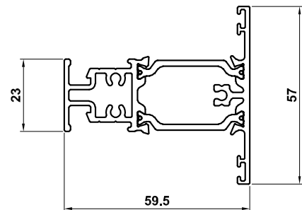
ETC4130 Transom/Mullion
