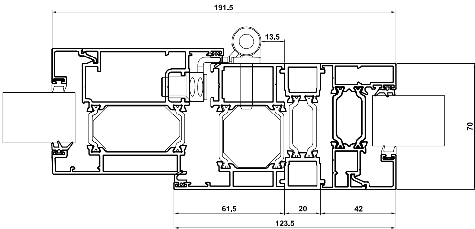
Flush Coupler
